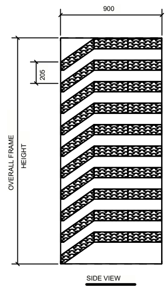
AL-900 LOUVRE FRAME
